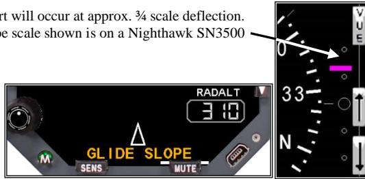
Figure 7-4 Generic GPWS Mode 5 Alert
