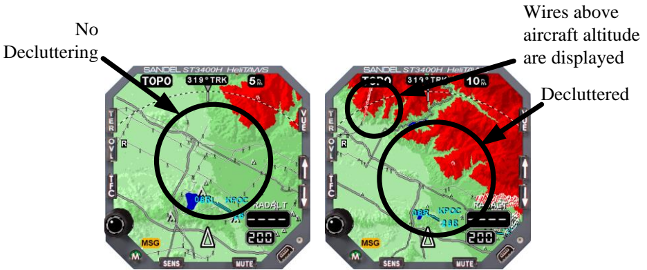
Figure 5-11 Decluttering
