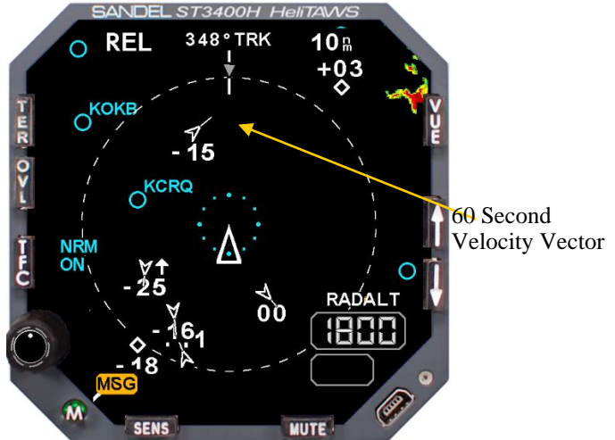
Figure 9-6 Targets with Velocity Vector
