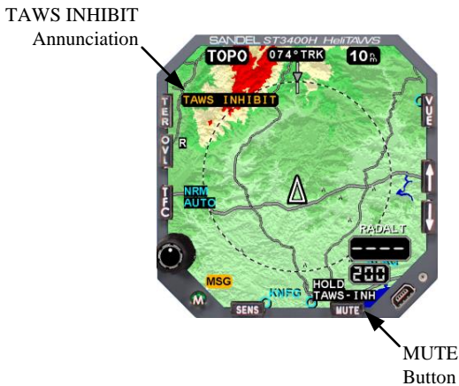
Figure 7-12 TAWS INHIBIT
