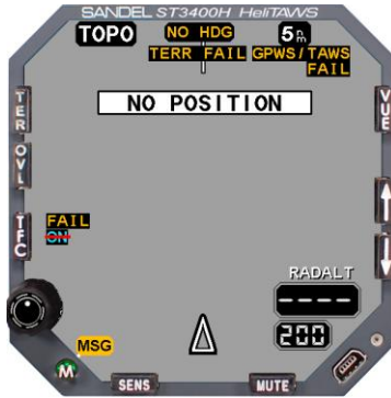
Figure 5-4 Initial Display
