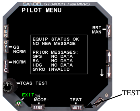
Figure 10-5 TEST
