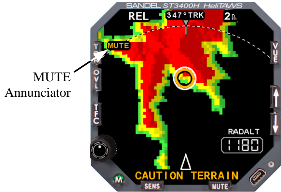
Figure 5-18 MUTE Annunciator
