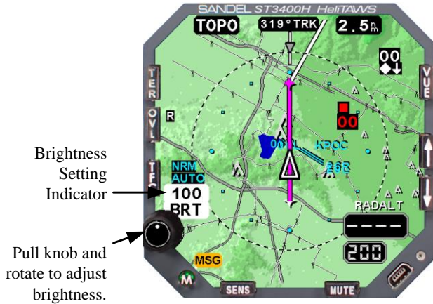
Figure 5-19 Brightness
