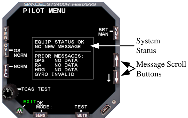
Figure 10-8 System Status
