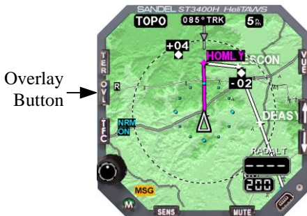
Figure 5-12 Overlay Button
