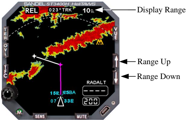
Figure 5-10 Display Ranging
