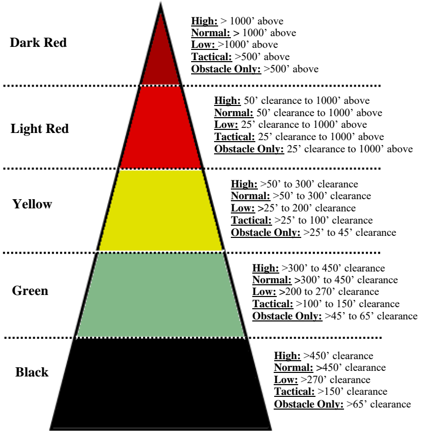
Figure 5-8 REL Display Color Banding Relative to aircraft altitude
