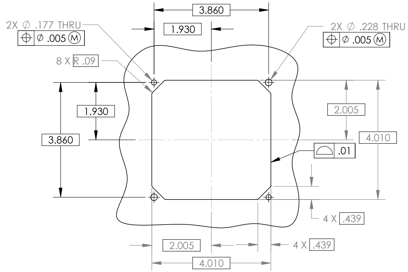
SUGGESTED PANEL CUT OUT (REF. ARINC SPECIFICATION 408A)
