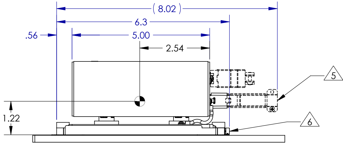
SIDE VIEW
