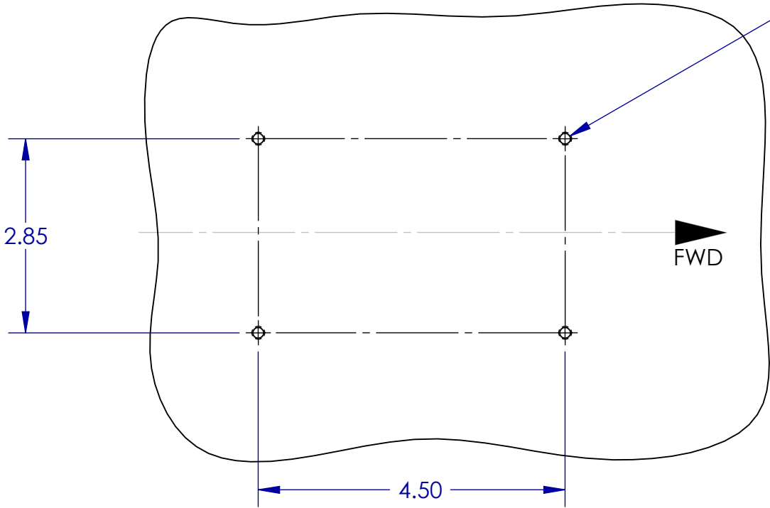
MOUNTING HOLE PATTERN 2
