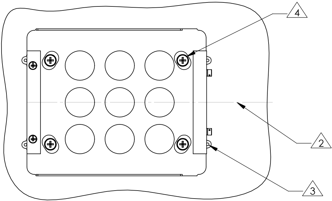
84051 MOUNTING PLATE INSTALLATION 2 3 4
